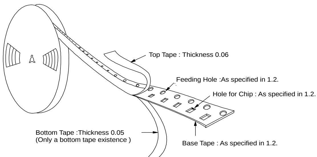
Fig.3 Taping Diagram
