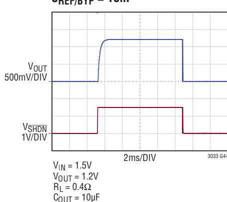
SHDN Transient Response C_{\text{REF/BYP}} = 10\text{nF}
