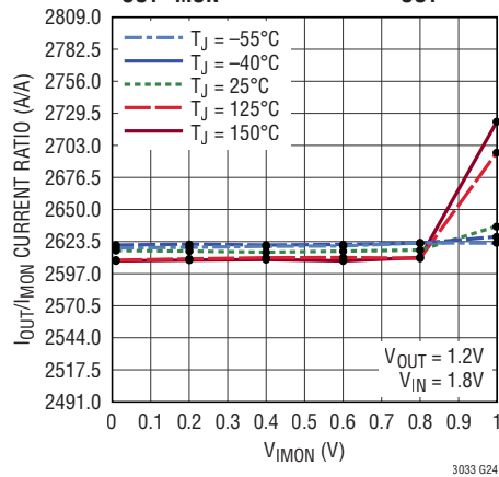
I_{\text{OUT}}/I_{\text{MON}} Current Ratio, I_{\text{OUT}} = 3\text{A}
