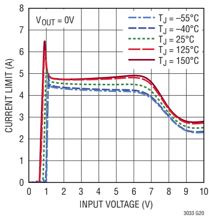
Internal Current Limit
