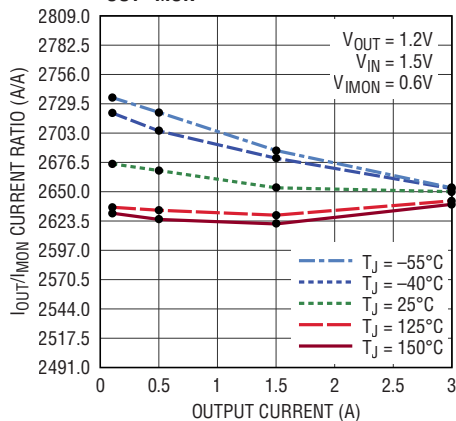
I_{\text{OUT}}/I_{\text{MON}} Current Ratio
