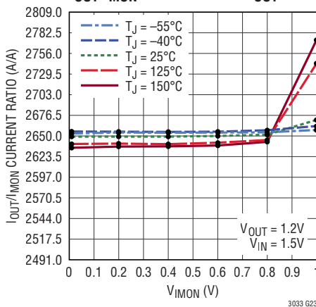
I_{\text{OUT}}/I_{\text{MON}} Current Ratio, I_{\text{OUT}} = 3\text{A}
