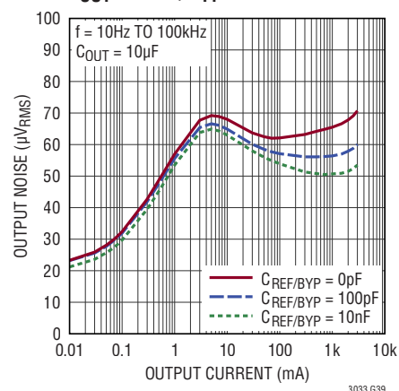
RMS Output Noise V_{\text{OUT}} = 0.2\text{V} , C_{\text{FF}} = 0
