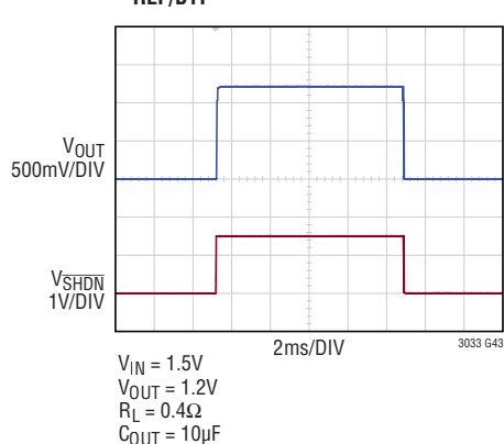
SHDN Transient Response C_{\text{REF/BYP}} = 0
