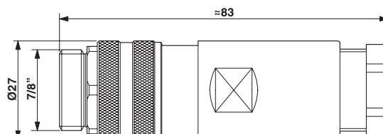
Dimensional drawing
