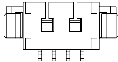
4 4極以上ロック形状 (2ロック) FIGURE OF MORE THAN 4 CIRCUIT (2 LOCKS)
