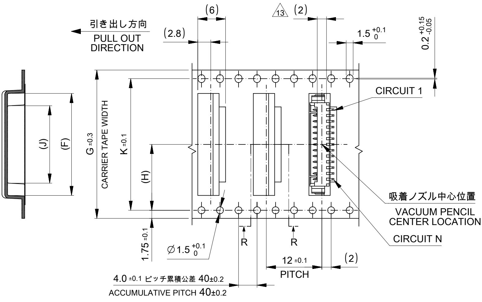
32mm幅(11~13極用)および44mm幅(14~15, 17極用)キャリアテープ 32mm (FOR 11~13 CIRCUIT) OR 44mm (FOR 14~15, 17 CIRCUIT) WIDTH CARRIER TAPE
