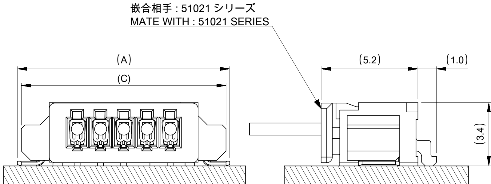
嵌合図 MATED CONNECTOR
