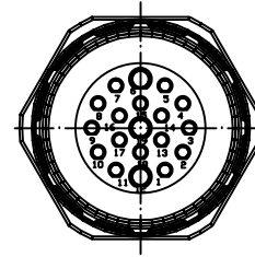
19-Pole (16+3)
