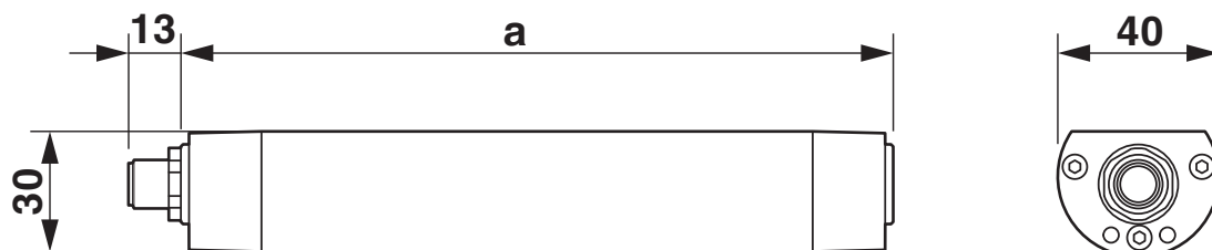
Dimensional drawing
