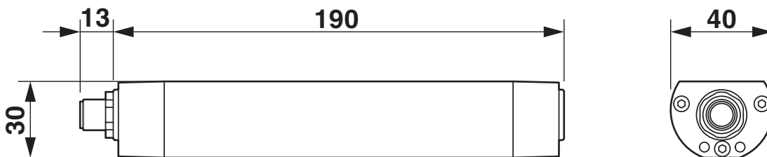
Dimensional drawing
