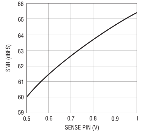
SNR vs SENSE, f IN = 5MHz, -1dB
