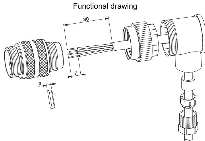
Schematic diagram
