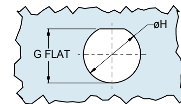
RECOMMENDED PANEL CUTOUT FOR STYLE 00 FRONT MOUNT JAM NUT
