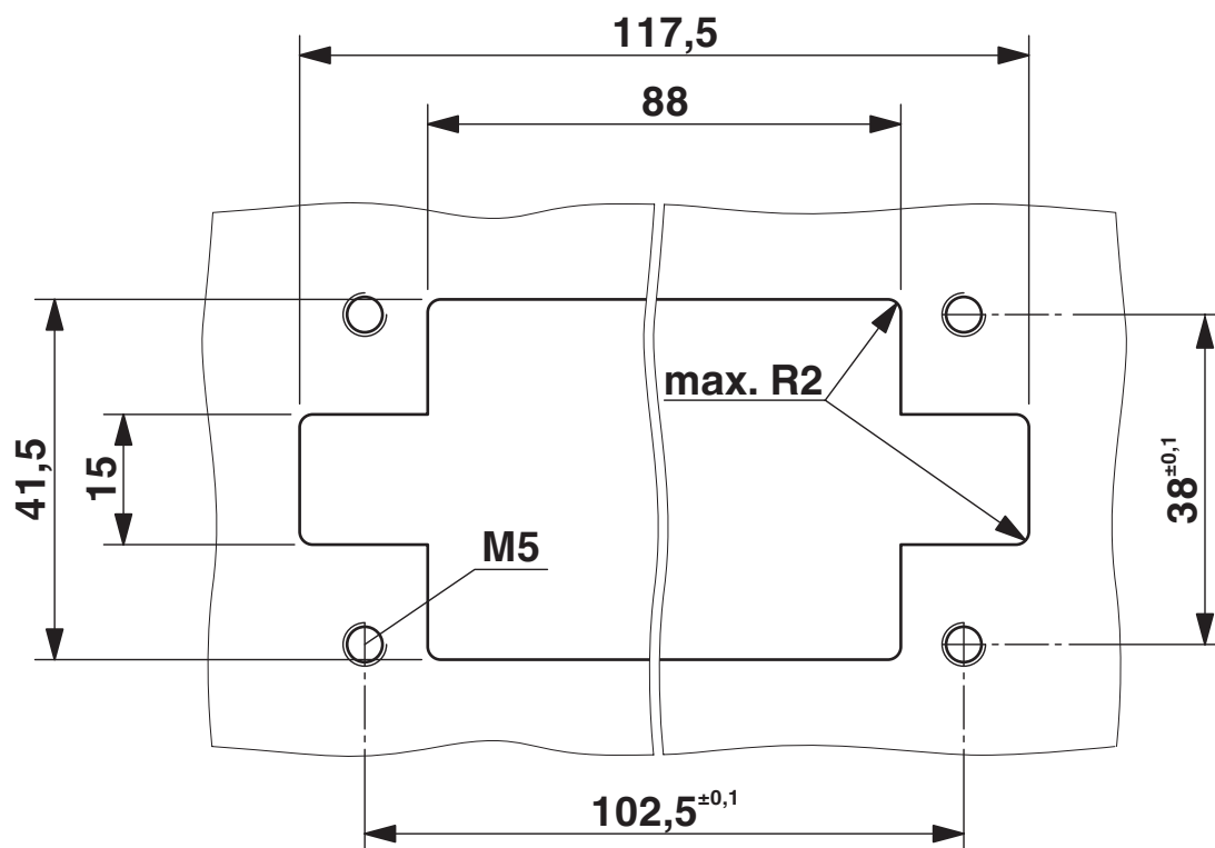
Dimensional drawing
