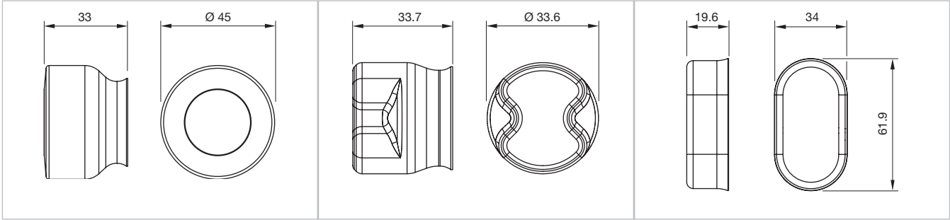
Dimensions [mm] for Part No. 45-543.1K00
