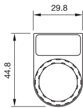
Dimensions [mm] for Part No. 45-564.1102
