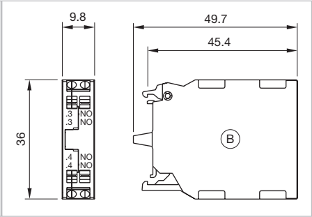
Dimensions [mm] B = Spring-type terminal for Part No. 45-313.1Z40, 45-313.1X40
