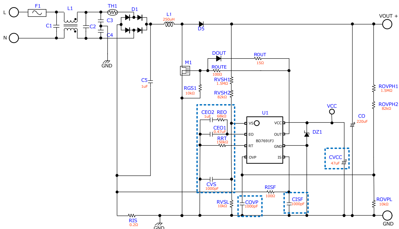
Figure 26. Parts placement
