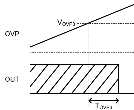
Figure 10. Timing chart
