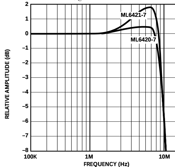
Figure 2b. Pass-Band Amplitude vs Frequency ( f_C = 9.3\text{MHz} ).
