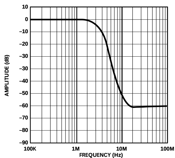
Figure 1d. Stop-Band Amplitude vs Frequency ( f_C = 3.0\text{MHz} ).
