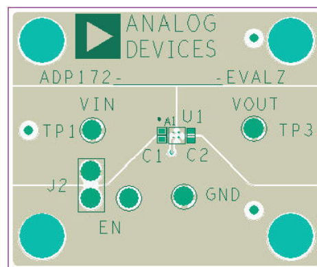
Figure 37. Example ADP172 PCB Layout
