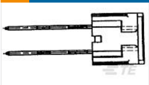
TE Part #1734290-1 IEEE 1394, RCPT, 6P, V/T, DIP, H 2.69
