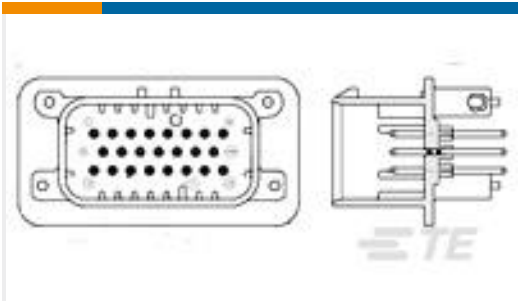
TE Part #1-776228-1 23POS,PIN DIA 1.3,HDR ASSY, 180DEG,COD 1
