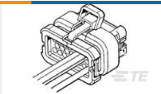
TE Part #770680-3 23POS,AMPSEAL,SOC HSG ASSY,SLD, COD 1
