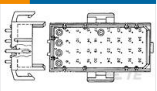
TE Part #640502-1 12P MR HDR ASSY V0
