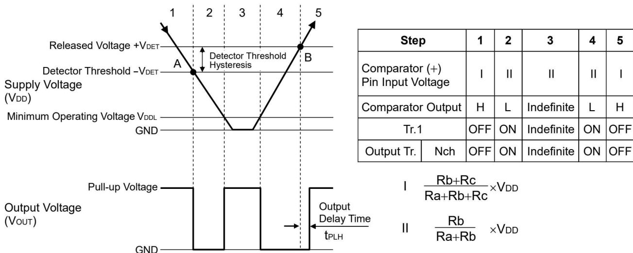
Operation Diagram
