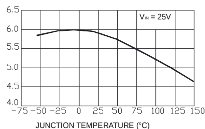
Oscillator Frequency
