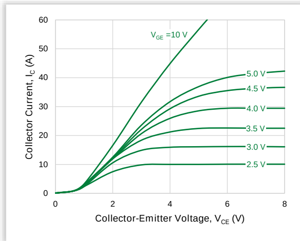
Figure 3. Output Characteristics ( T_J = 150^\circ\text{C} )
