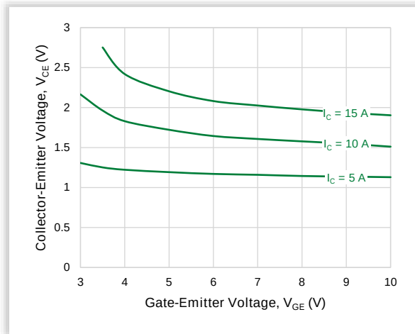
Figure 7. Collector-Emitter Voltage vs. Gate-Emmitter Voltage ( T_J = 150^\circ\text{C} )
