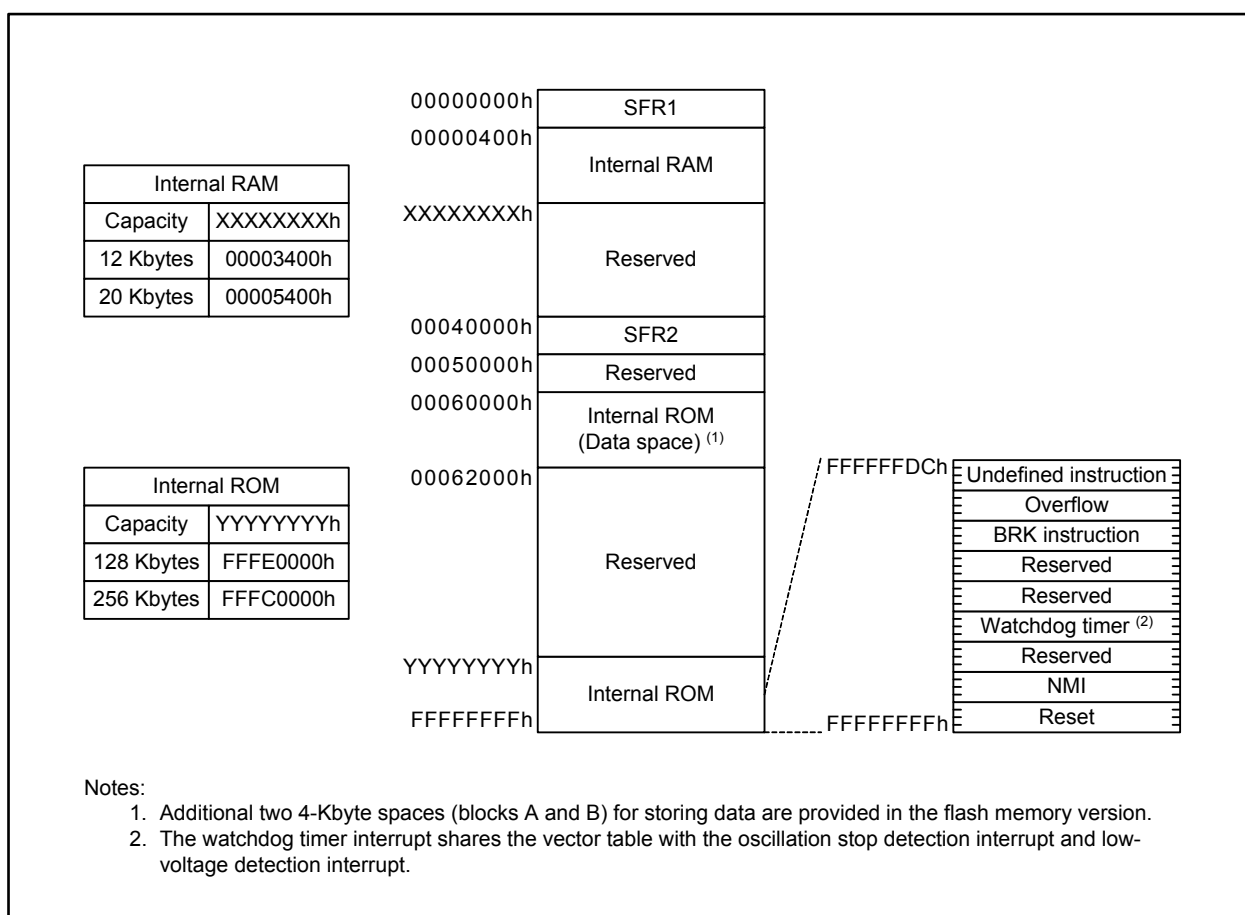
Figure 3.1 Memory Mapping
