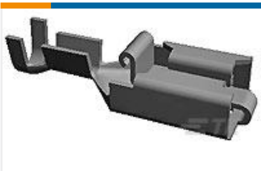
TE Part #927855-6 PL RECEPTACLE 1.0-2.5 MM2 PTP CUSN 30
