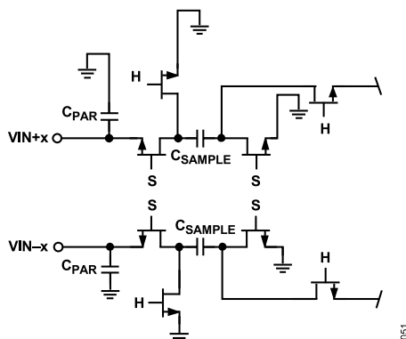
Figure 54. Switched-Capacitor Input Circuit
