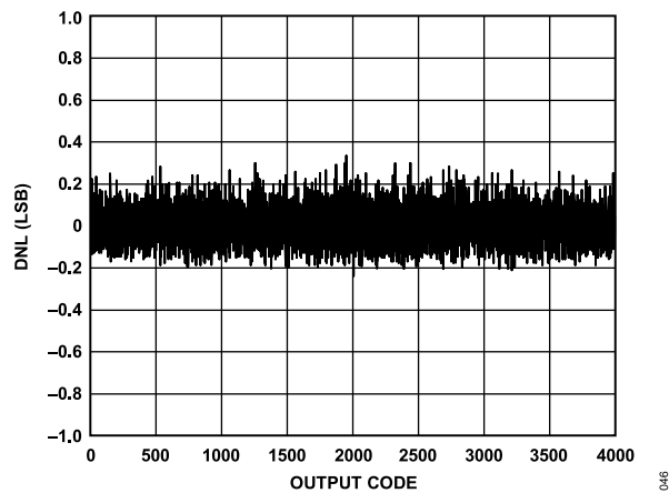
Figure 41. DNL, f_{IN} = 9.7 MHz, f_{SAMPLE} = 125 MSPS
