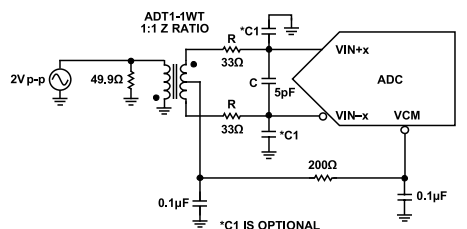
Figure 58. Differential Transformer-Coupled Configuration for Baseband Applications
