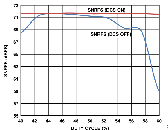
Figure 63. SNR vs. DCS On/Off
