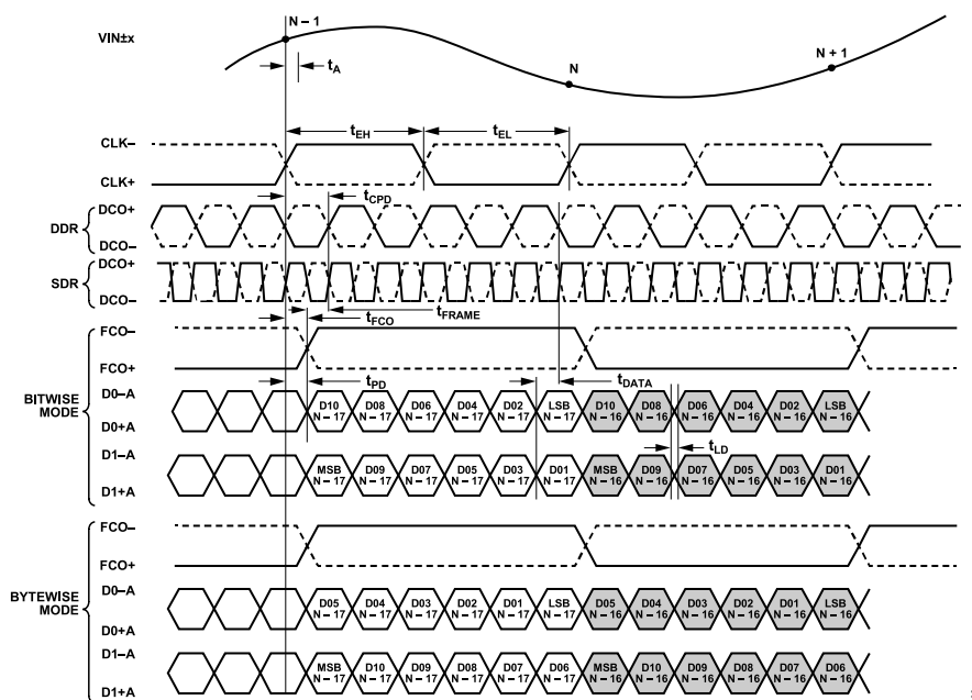
Figure 4. 12-Bit DDR/SDR, Two-Lane, 2x Frame Mode
