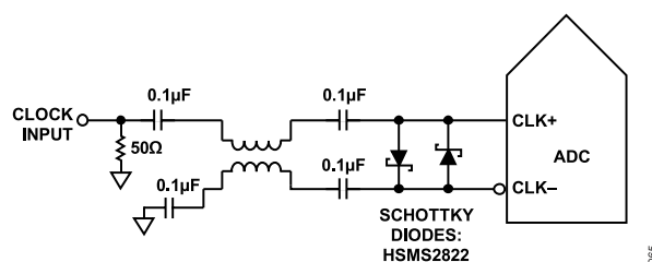
Figure 62. Balun-Coupled Differential Clock (Up to 1 GHz)
