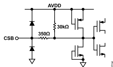
Figure 52. Equivalent CSB Input Circuit
