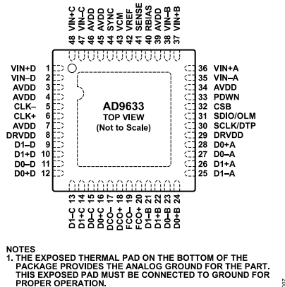
Figure 9. 48-Lead LFCSP Pin Configuration, Top View
