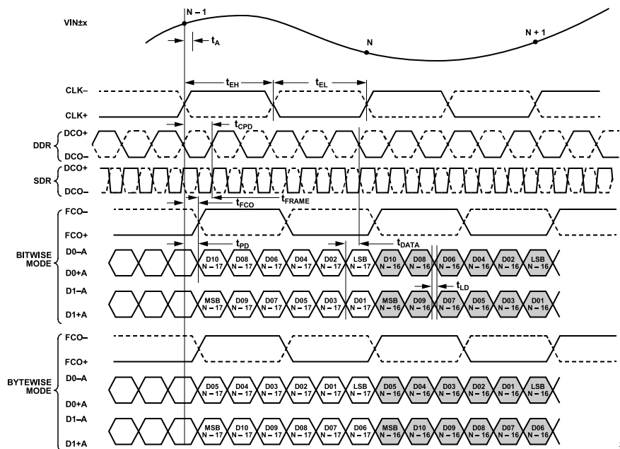
Figure 2. 12-Bit DDR/SDR, Two-Lane, 1x Frame Mode (Default)
