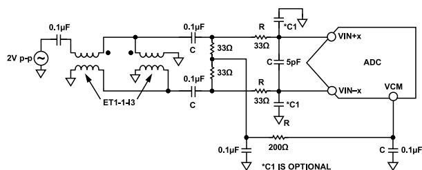
Figure 57. Differential Double Balun Input Configuration for Baseband Applications
