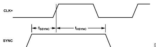
Figure 8. SYNC Input Timing Requirements
