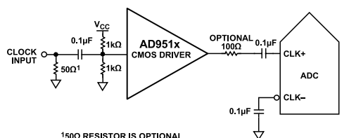
Figure 66. Single-Ended 1.8 V CMOS Input Clock (Up to 200 MHz)
