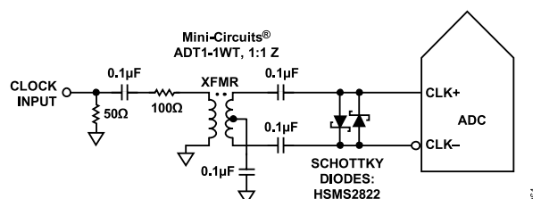
Figure 61. Transformer-Coupled Differential Clock (Up to 200 MHz)
