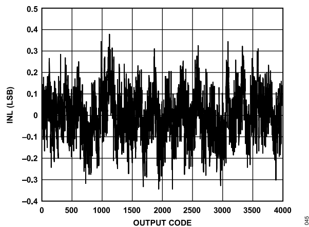
Figure 40. INL, f_{IN} = 9.7 MHz, f_{SAMPLE} = 125 MSPS
