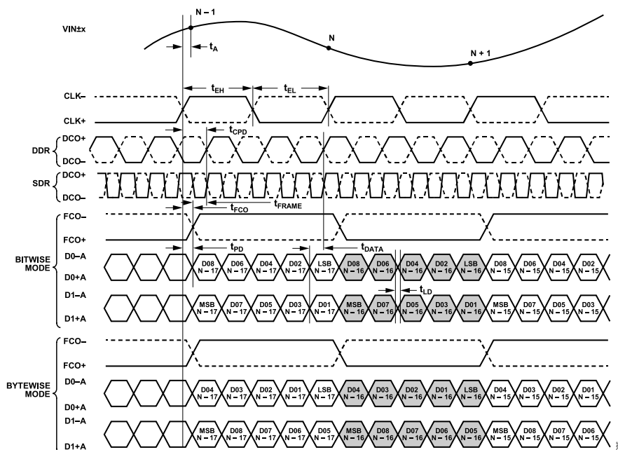
Figure 5. 10-Bit DDR/SDR, Two-Lane, 2x Frame Mode
