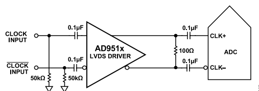
Figure 65. Differential LVDS Sample Clock (Up to 1 GHz)
