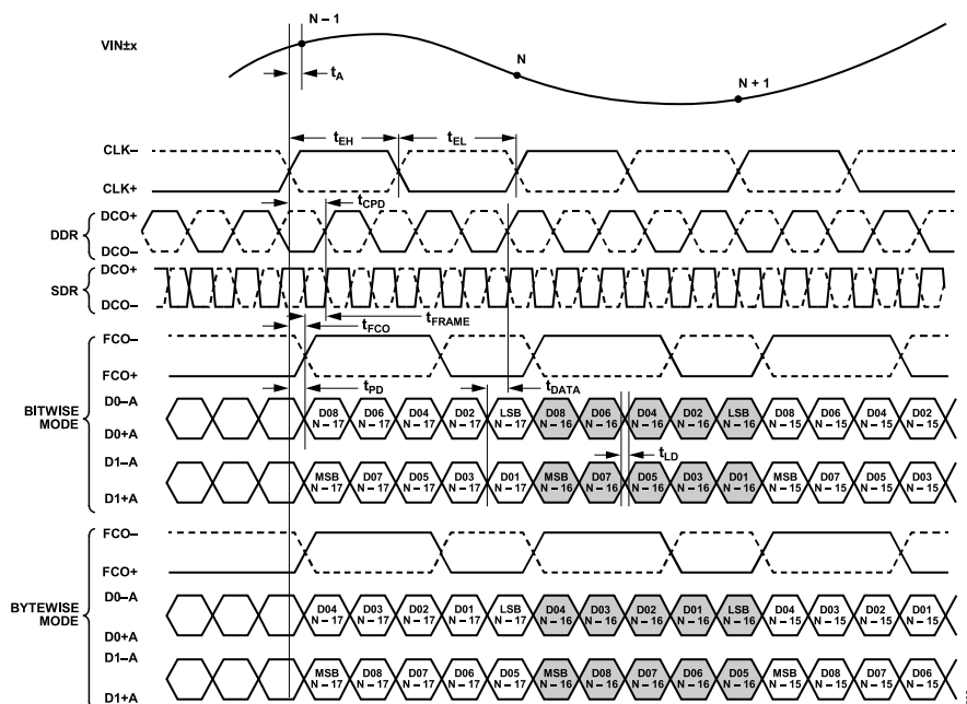
Figure 3. 10-Bit DDR/SDR, Two-Lane, 1x Frame Mode
