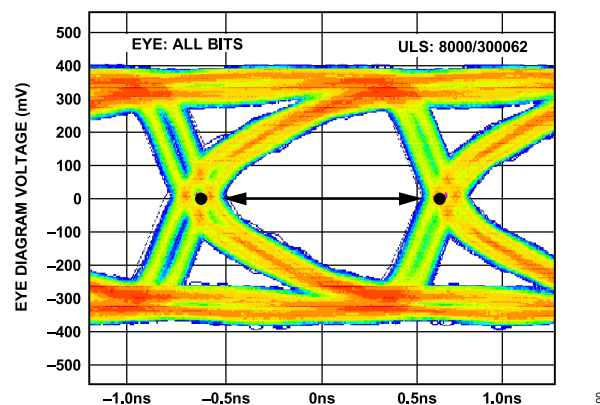
Figure 71. Data Eye for LVDS Outputs in ANSI-644 Mode with Trace Lengths Less than 24 Inches on Standard FR-4 Material, External 100 \Omega Far-End Termination Only
