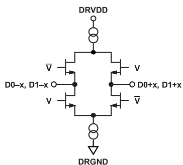
Figure 49. Equivalent Digital Output Circuit
