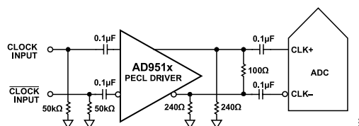
Figure 64. Differential PECL Sample Clock (Up to 1 GHz)
