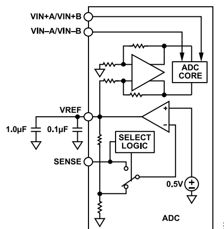
Figure 56. Internal Reference Configuration
