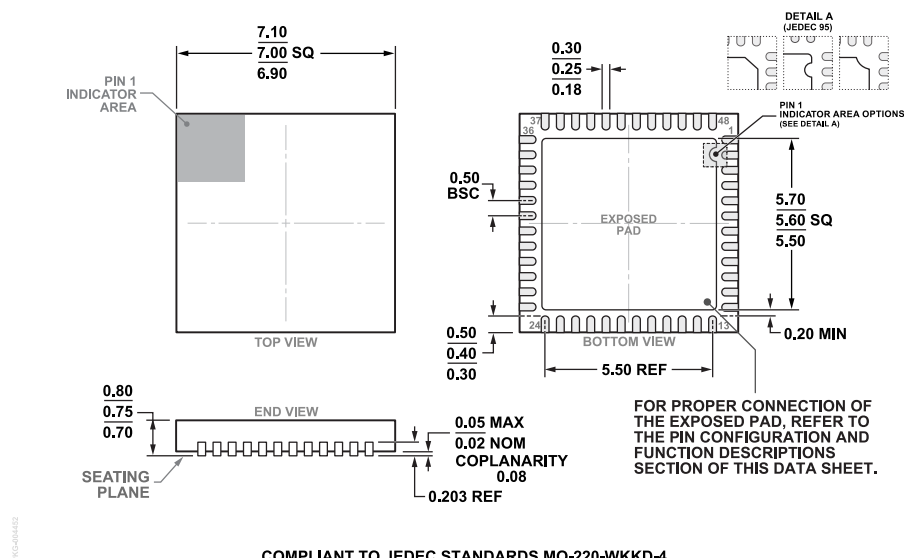
Figure 78. 48-Lead Lead Frame Chip Scale Package [LFCSP] 7 mm × 7 mm Body and 0.75 mm Package Height (CP-48-13) Dimensions shown in millimeters
