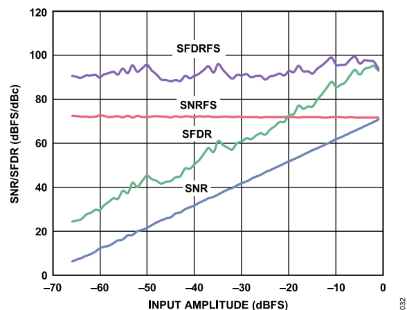
Figure 35. SNR/SFDR vs. Analog Input Level, f_{IN} = 9.7 MHz, f_{SAMPLE} = 125 MSPS
