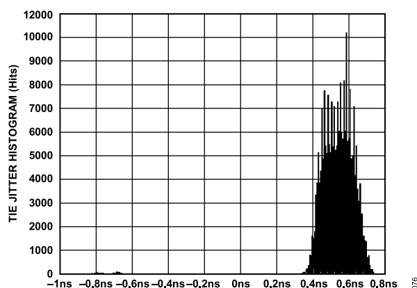
Figure 74. Time Interval Error (TIE) Jitter Histogram for LVDS Outputs in ANSI-644 Mode with Trace Lengths Greater than 24 Inches on Standard FR-4 Material, External 100 \Omega Far-End Termination Only
