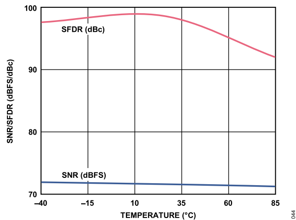
Figure 39. SNR/SFDR vs. Temperature, f_{IN} = 10.3 MHz, f_{SAMPLE} = 125 MSPS
