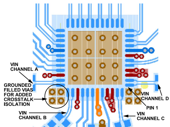
Figure 77. Layout Technique to Maximize Crosstalk Performance
