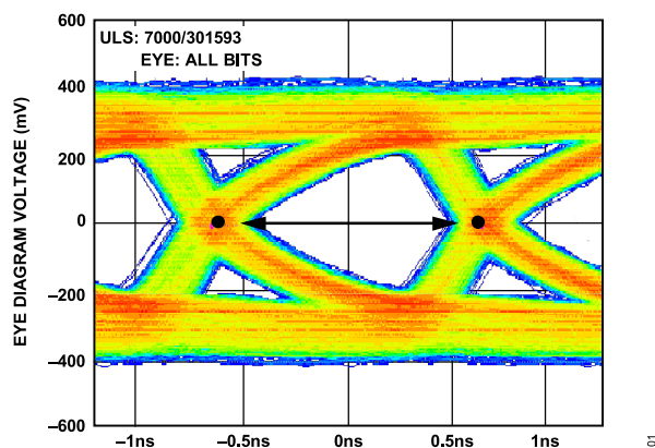
Figure 73. Data Eye for LVDS Outputs in ANSI-644 Mode with Trace Lengths Greater than 24 Inches on Standard FR-4 Material, External 100 \Omega Far-End Termination Only
