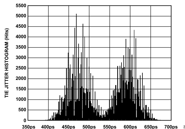
Figure 72. Time Interval Error (TIE) Jitter Histogram for LVDS Outputs in ANSI-644 Mode with Trace Lengths Less than 24 Inches on Standard FR-4 Material, External 100 \Omega Far-End Termination Only
