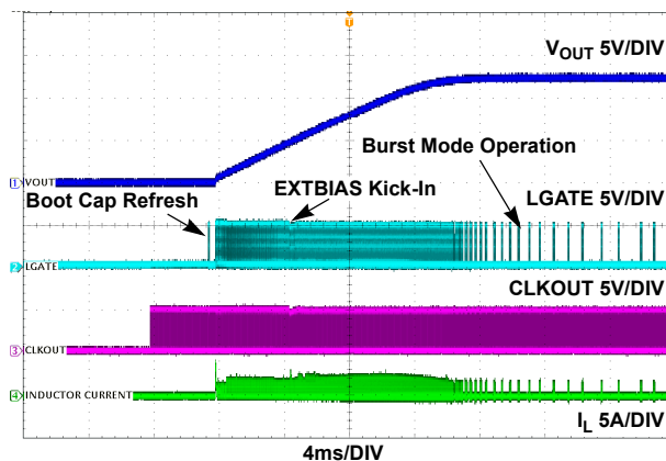
Figure 23. Start-Up Waveforms; Mode = DEM, Load = 0A, V_{IN} = 48V
