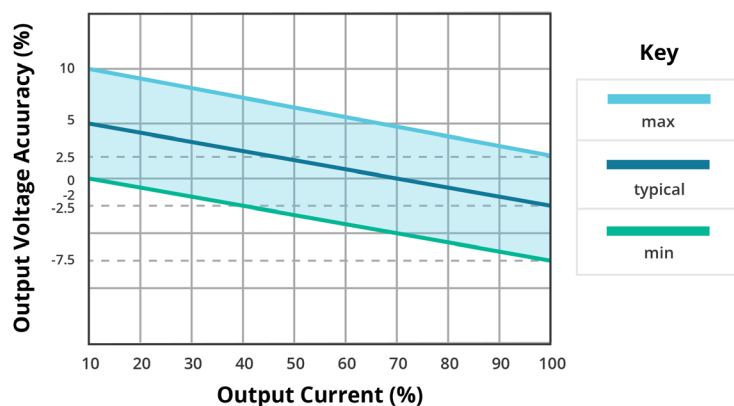
OUTPUT REGULATION CURVE
