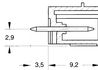
B73N3V (vertical solder pins)
