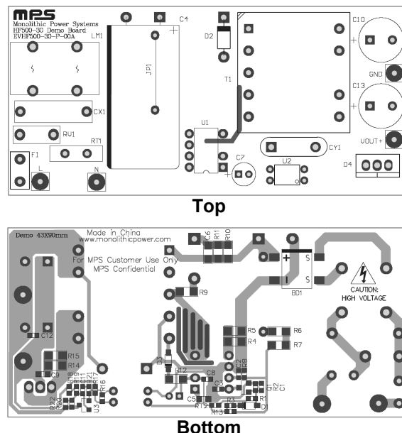
Figure 13: Recommended PCB Layout
