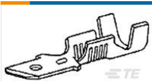
TE Part #60850-2 187 FASTON REC 18-14 AWG TPBR
