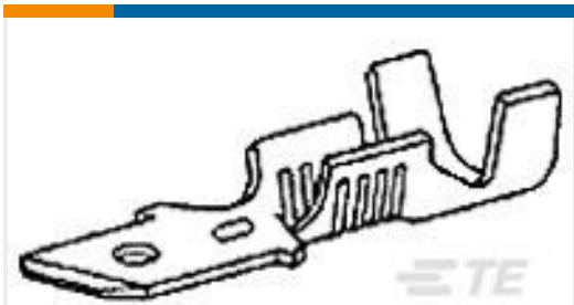
TE Part #61687-2 187 FASTON TAB 18-14 AWG TPBR
