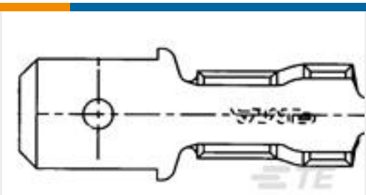
TE Part #41412 FASTON 250(6.3MM) TAB 18-14 AWG TPBR
