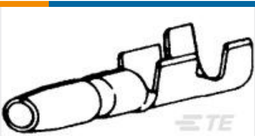
TE Part #60766-2 SHUR PLUG .156 18-14 AWG PTPBR
