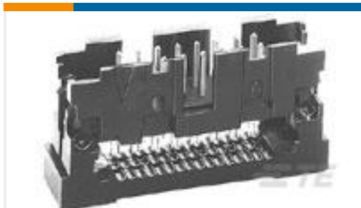
TE Part #1-111446-5 14 UNIV I/O, NO EARS,LEAD FREE
