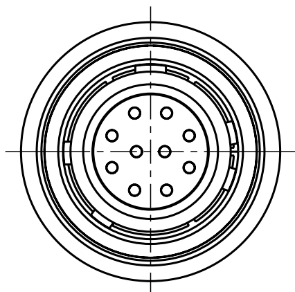
S1AYBR-P10XFG0-0000 Mechanical coding: B Color coding: red
