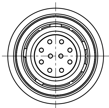
S1AYDR-P10XFG0-0000 mechanical coding: D Color coding: green
