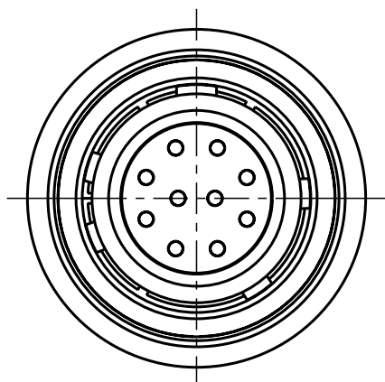
S1AYCR-P10XFG0-0000 mechanical coding: C Color coding: blue
