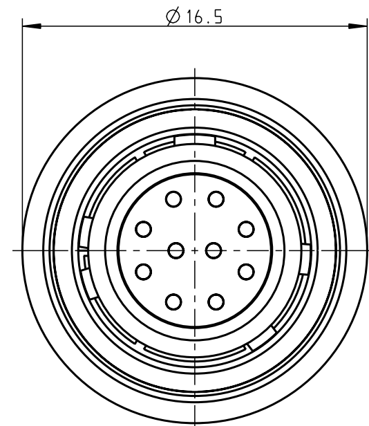
S1AYAR-P10XFG0-0000 Mechanical coding: A Color coding: light brown
