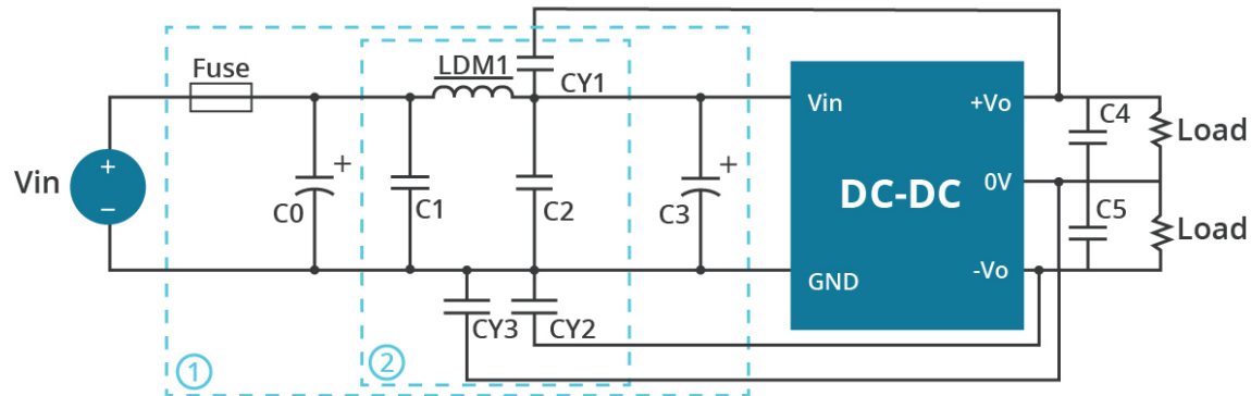
Figure 4 Dual output
