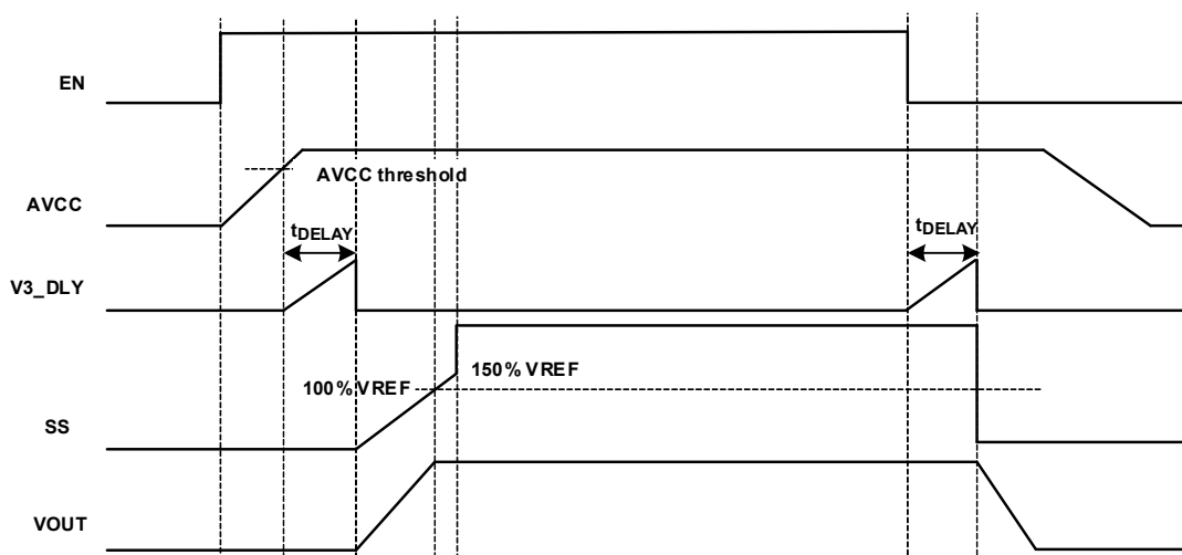
Figure 63. Delay Function
