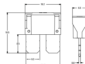
Dimensions [mm]
