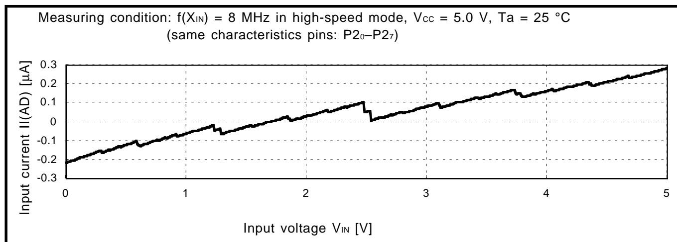
Fig. 3.2.74 V_{IN} -II(AD) characteristics (A-D port input current during A-D conversion, f(X_{IN}) = 8 MHz in high-speed mode: One Time PROM version)
