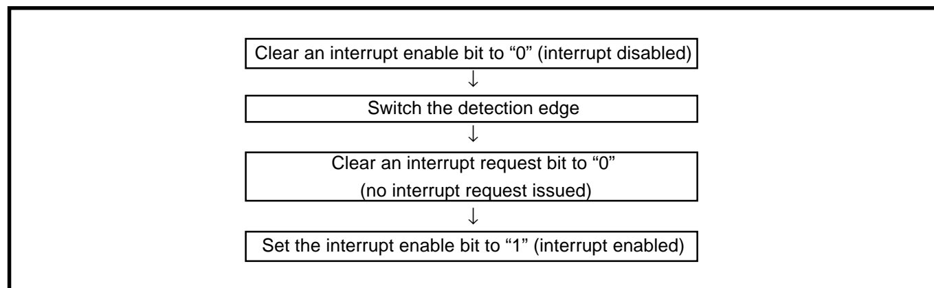
Fig. 3.3.5 Sequence of switch the detection edge
