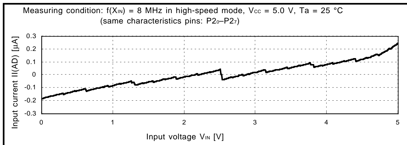
Fig. 3.2.31 V_{IN} - I(AD) characteristics (A-D port input current during A-D conversion, f(X_{IN}) = 8 MHz in high-speed mode: Mask ROM version)
