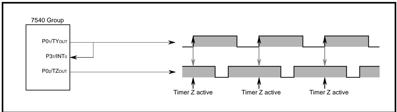
Fig. 2.5.39 Example of waveform generation and peripheral circuit
