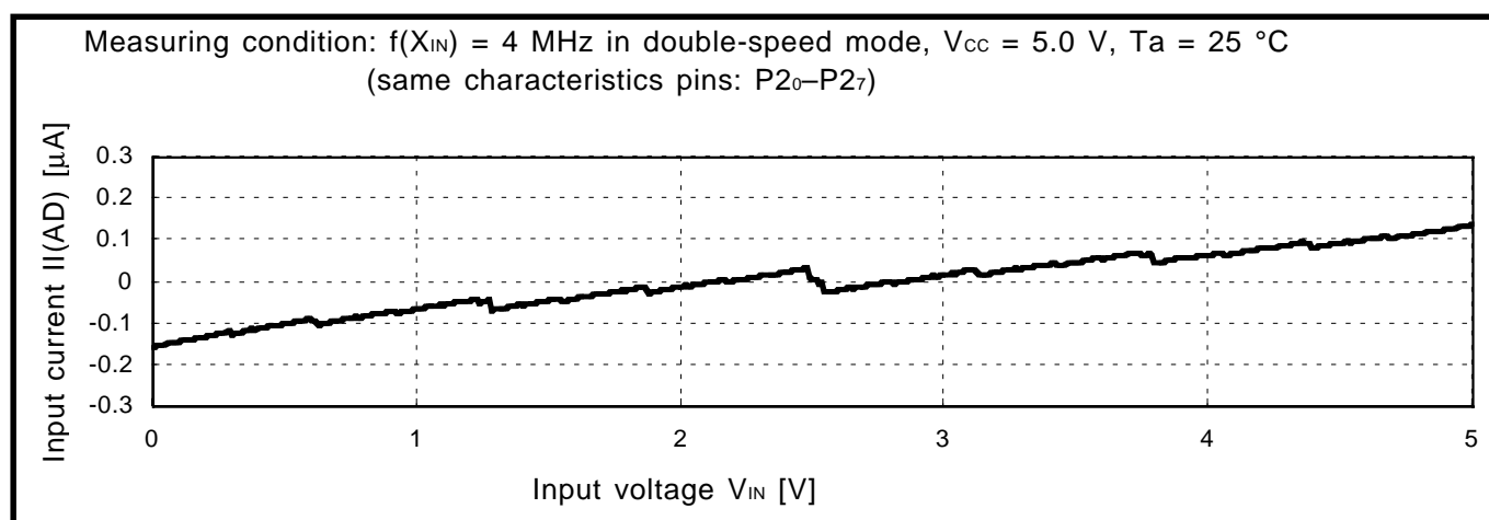
Fig. 3.2.76 V_{IN} -II(AD) characteristics (A-D port input current during A-D conversion, f(X_{IN}) = 4 MHz in double-speed mode: One Time PROM version)
