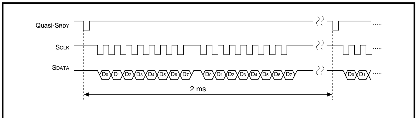
Fig. 2.7.10 Timing chart
