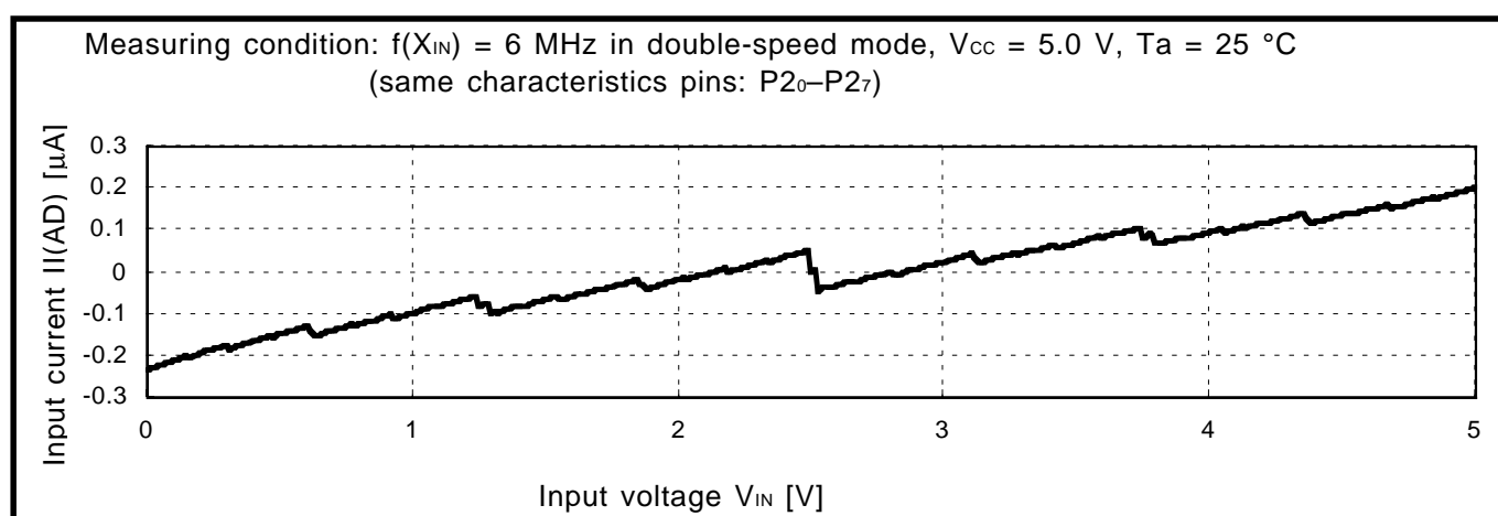
Fig. 3.2.75 V_{IN} -II(AD) characteristics (A-D port input current during A-D conversion, f(X_{IN}) = 6 MHz in double-speed mode: One Time PROM version)
