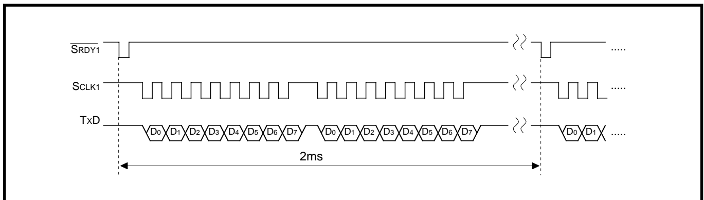
Fig. 2.6.13 Timing chart
