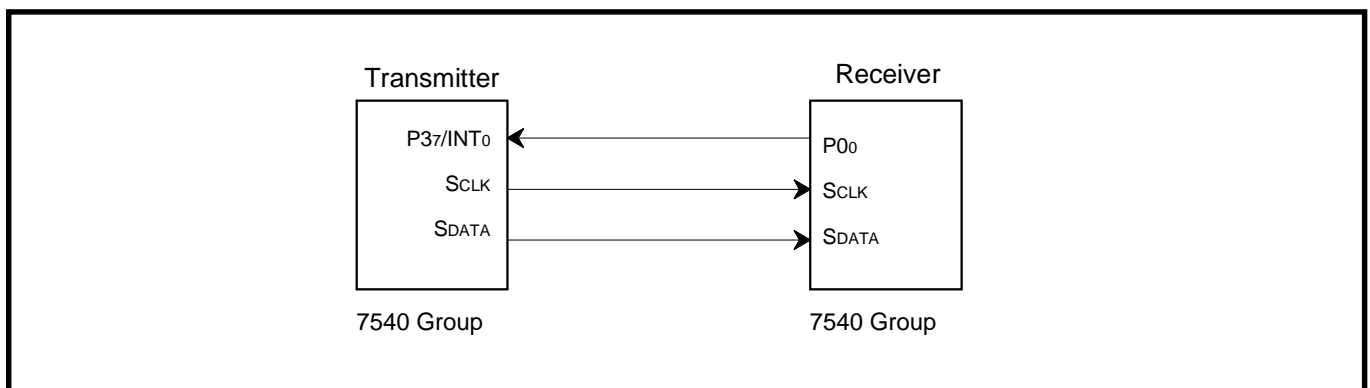
Fig. 2.7.9 Connection diagram
