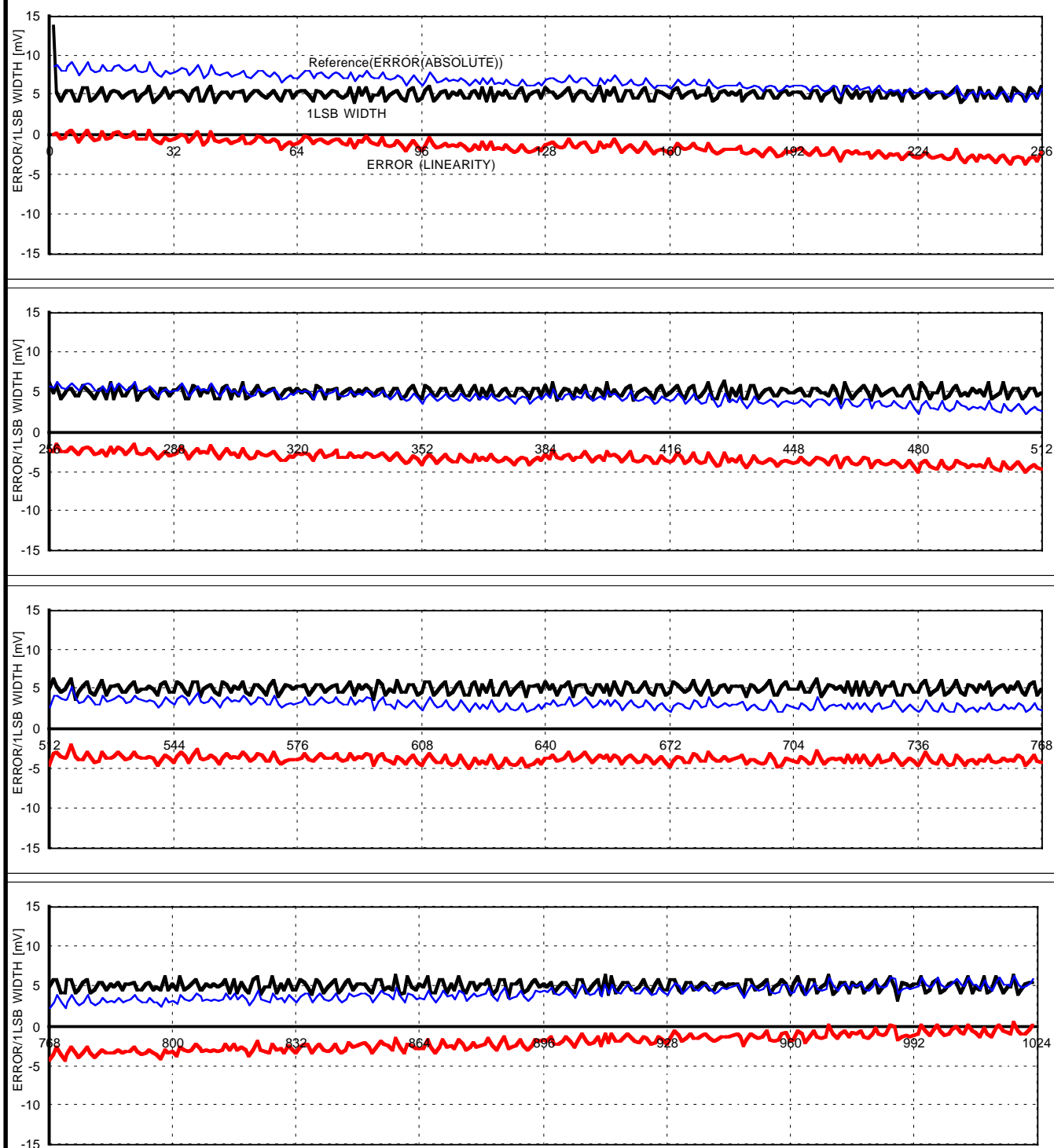
Fig. 3.2.41 A-D conversion accuracy typical characteristic example-1 (Mask ROM version)
