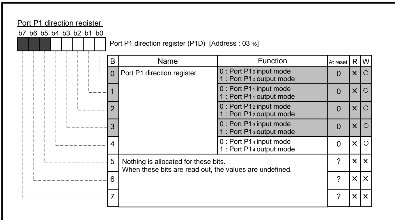
Fig. 2.4.3 Structure of Port P1 direction register
