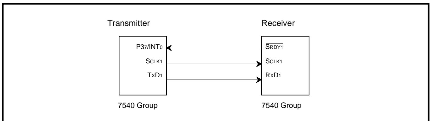
Fig. 2.6.12 Connection diagram
