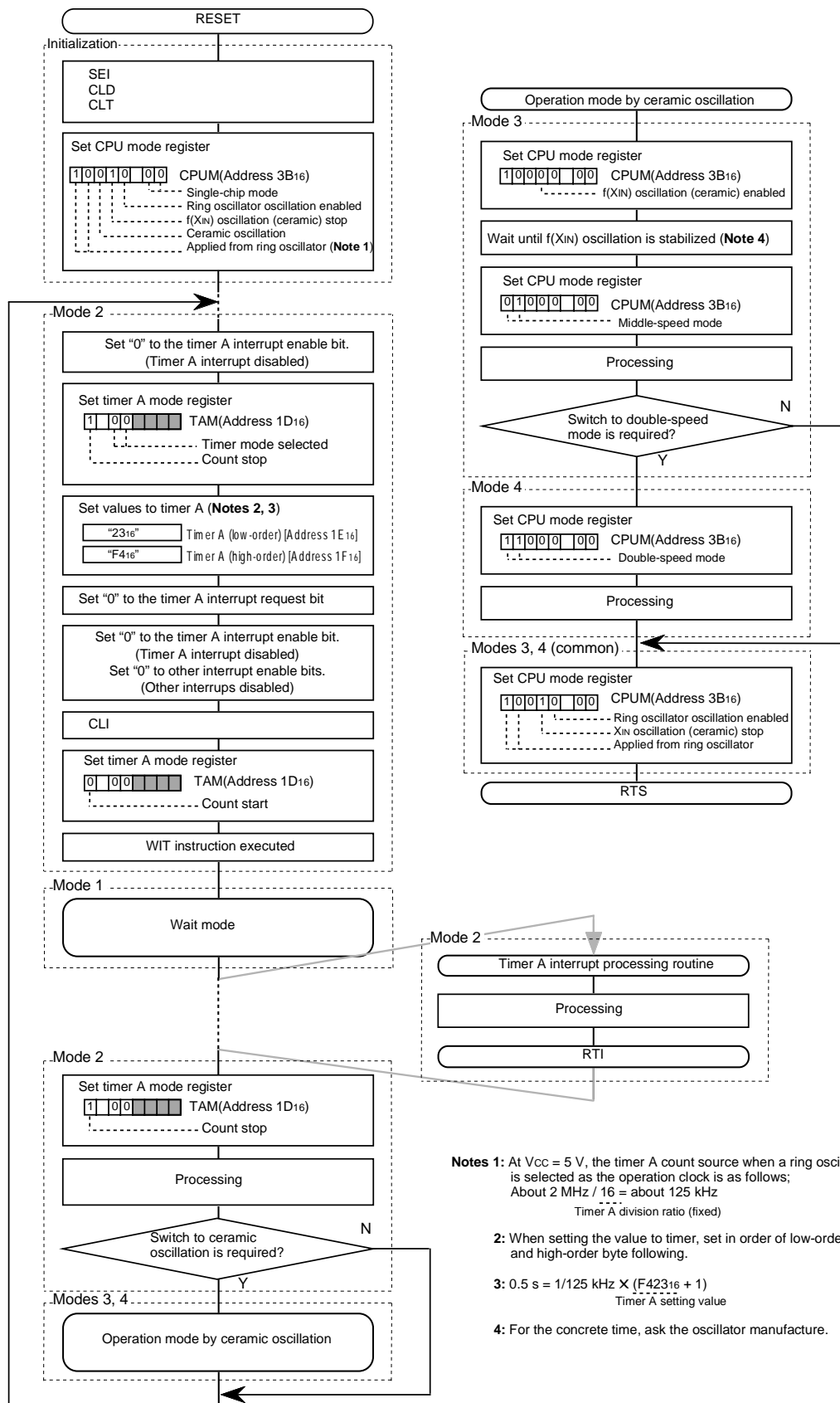
Fig. 2.9.11 Control procedure
