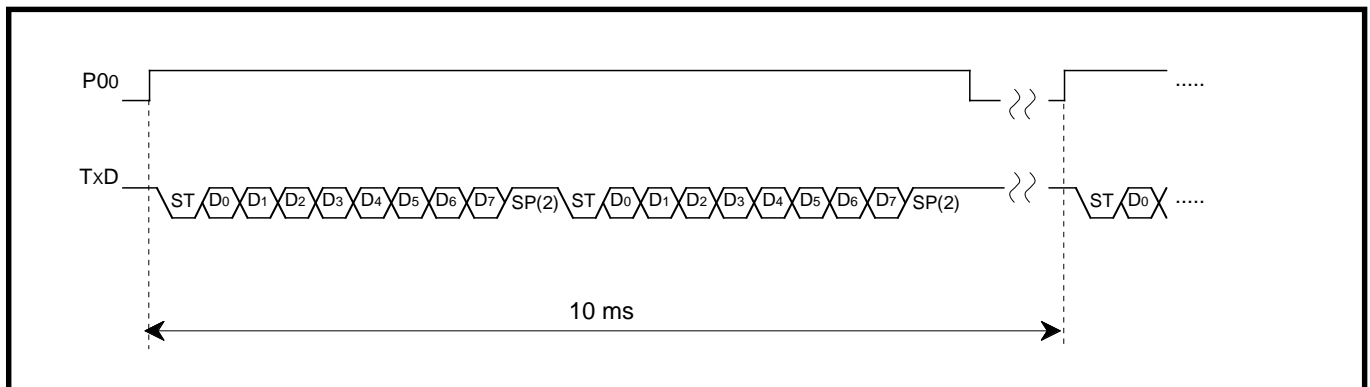
Fig. 2.6.19 Timing chart
