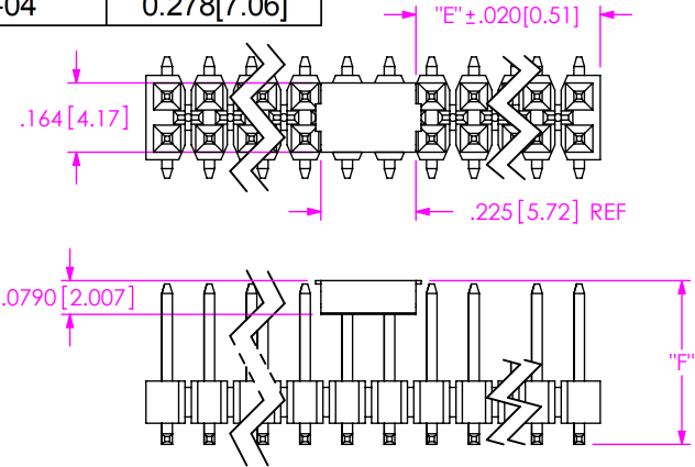
FIG 5 -M: METAL PICK AND PLACE PAD (DIFFERENT AS SHOWN, OTHERWISE SAME AS FIG 1) "E" = ((\text{NO OF POS} \times .100 [2.54]) - .225 [5.72]) / 2 NOTE: HAND FILL USE LMP-01 MACHINE FILL USE LMP-01
