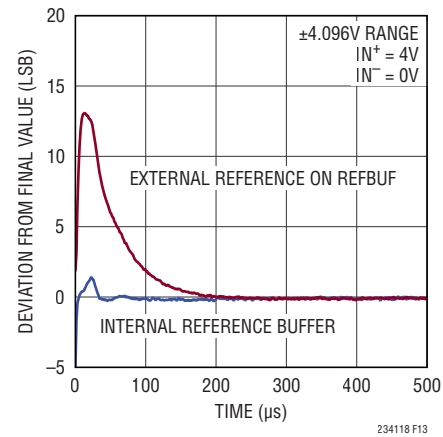
Figure 13. Burst Conversion Response of the LTC2341-18, f_{\text{SMPL}} = 666\text{ksps}
