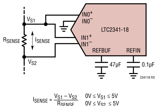
Figure 7. Simultaneously Sense Voltage (CH0) and Current (CH1) Over a Wide Common Mode Range
