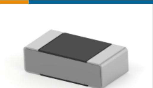
TE Part #3-1879130-3 RN 0402 3K4 0.1% 10PPM 5K RL
