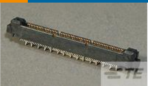
TE Part # 1-5767119-0 MICT,PLG,114,ASY,.025,TAPE PKG
