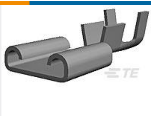
TE Part #6-160432-0 250 FASTON REC 20-16 AWG TPBZ
