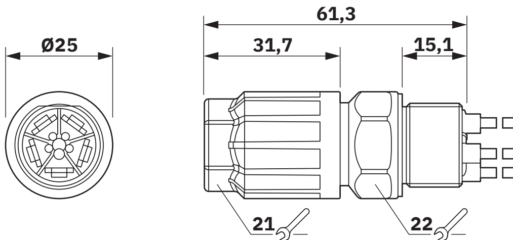
Dimensional drawing
