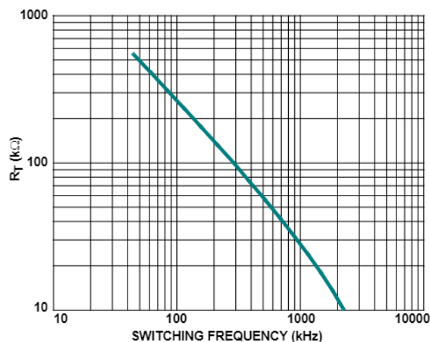
FIGURE 13. R_T vs SWITCHING FREQUENCY
