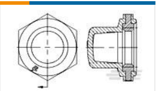
TE Part #1825615-1 BP1048004=Boot,Pushbutton
