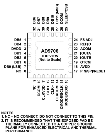
Figure 4. AD9706 Pin Configuration
