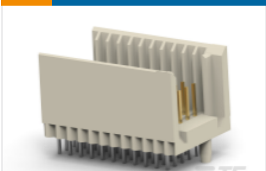
TE Part #5352128-1 Hard Metric Male Connector: Traditional Backplane, Mezzanine, 2mm
