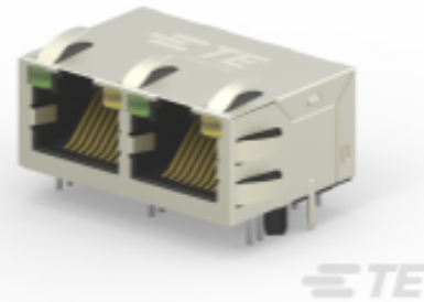
TE Part #2301996-5 RJ45 JACK INT.MAG. 10/100 LED 1X2 INV.
