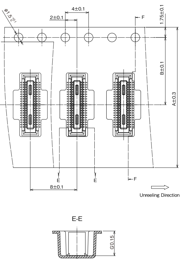
Embossed Tape Dimensions
