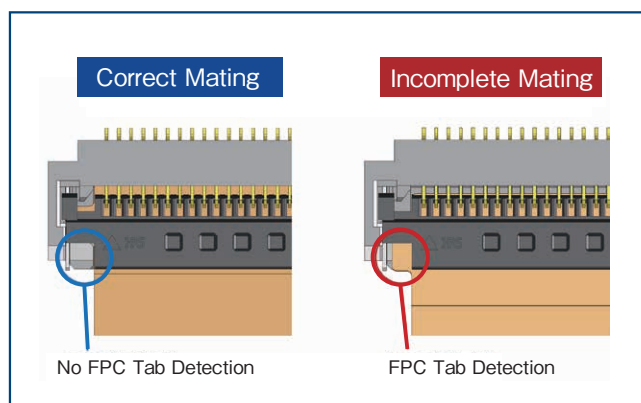
FPC/FFC Mis-Mating Detection
