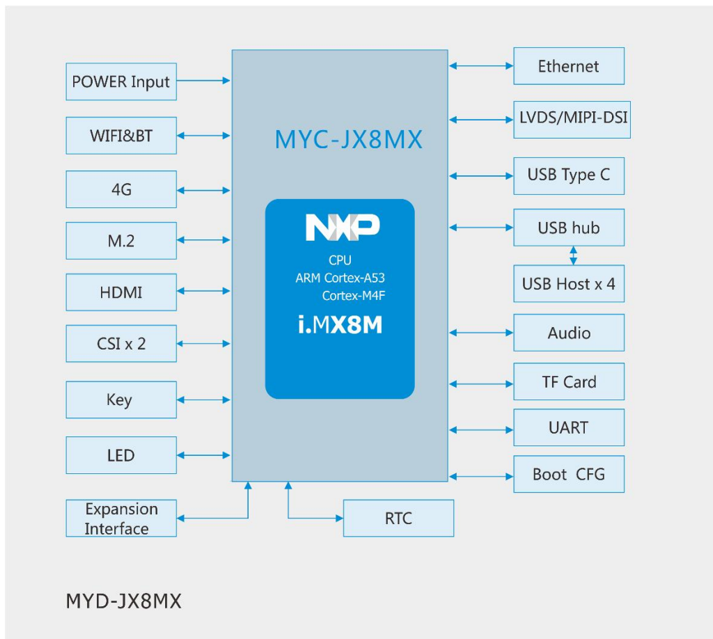
MYD-JX8MX Development Board Function Block Diagram
