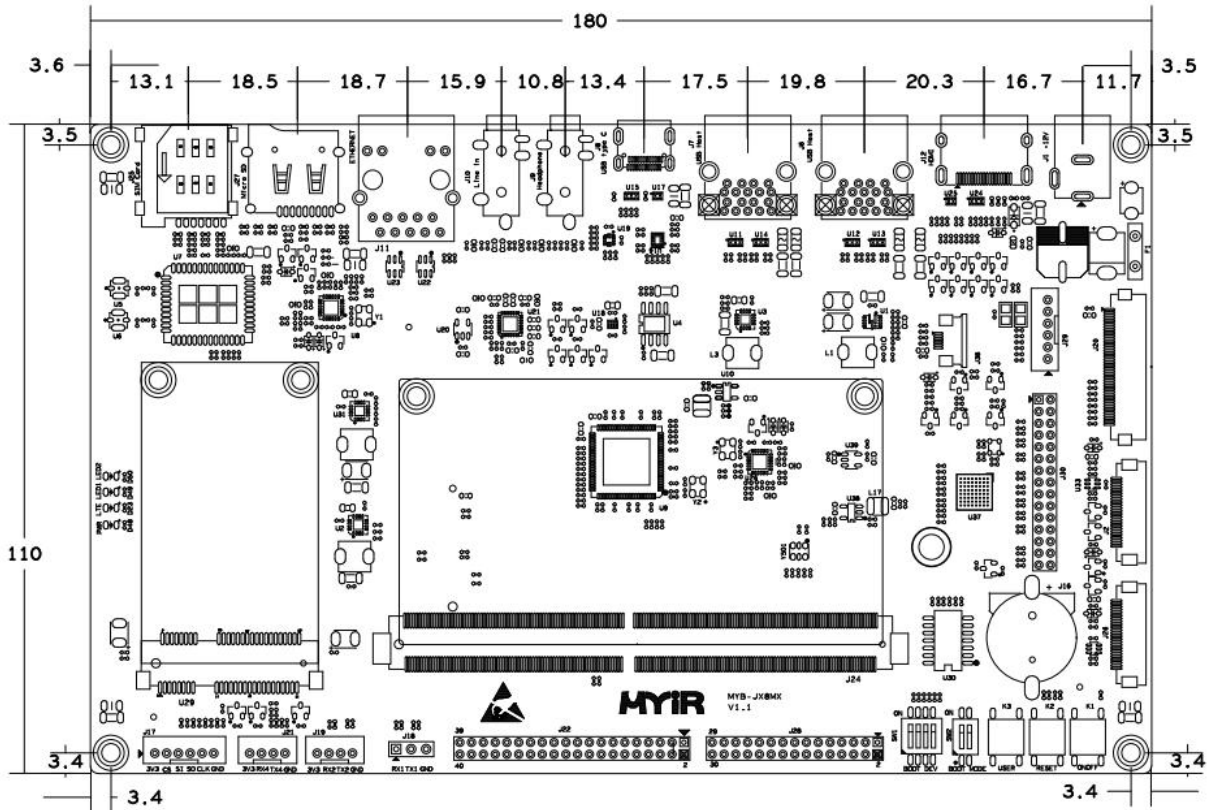
MYD-JX8MX Dimensions Chart
