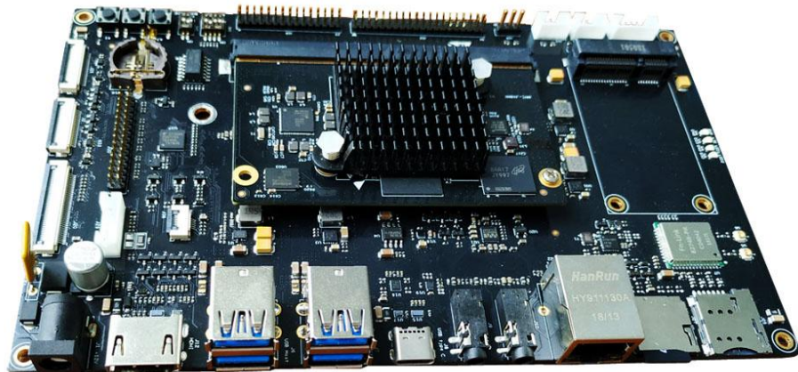
MYD-JX8MX Development Board
