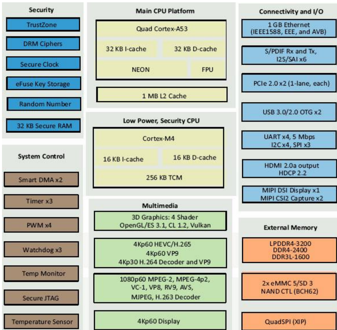
i.MX 8M System Block Diagram
