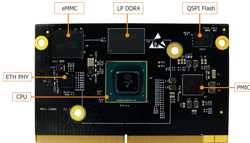
MYC-JX8MX CPU Module (delivered with installed heatsink by default)
