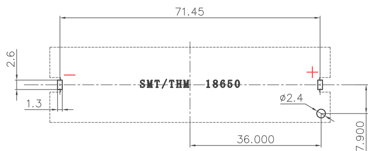
PCB Layout Diagram TOP View
