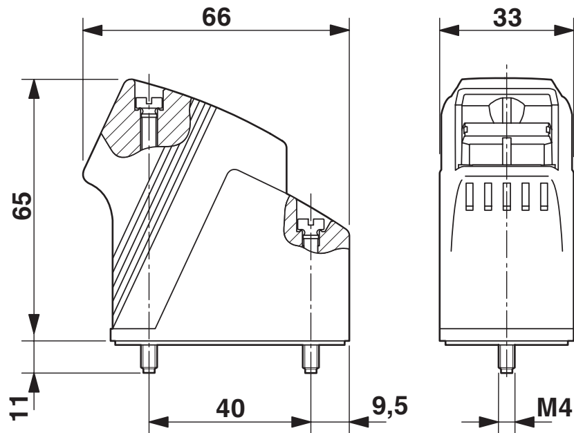
Dimensional drawing
