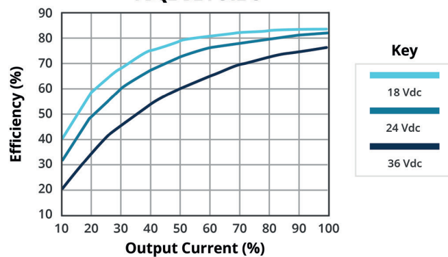
EFFICIENCY VS OUTPUT LOAD PDQ2-D24-S12-S
